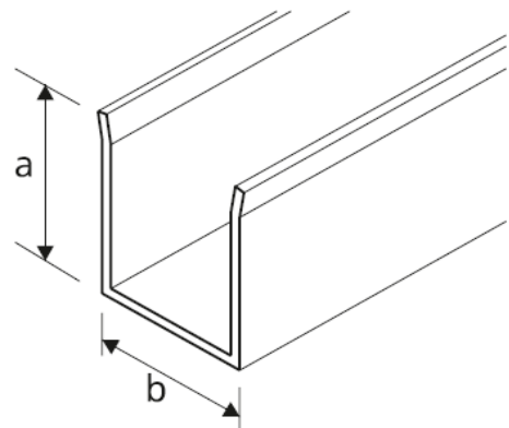
Galvanized steel guide (measures b x a: 18x22 mm or 18x32 mm)
