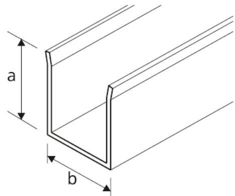
Galvanized steel guide (measures b x a: 18x22 mm or 18x32 mm)
